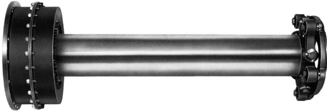
CENTALINK-joint with highly flexible CENTAX-coupling size 65 for ship main propulsion. MAN 2842 - 700 kW / 2300 rpm.
