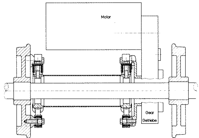
CENTALINK in axle drive of a rail car.
