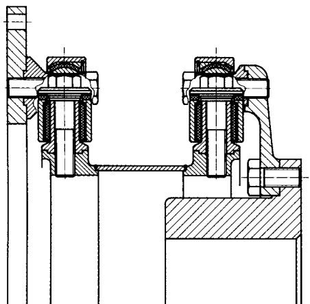
CENTALINK short version Kurzbauforn
