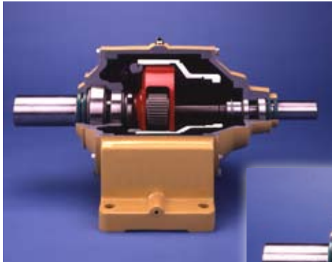
Single Reduction
