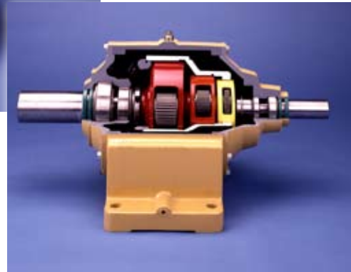
Triple Reduction
